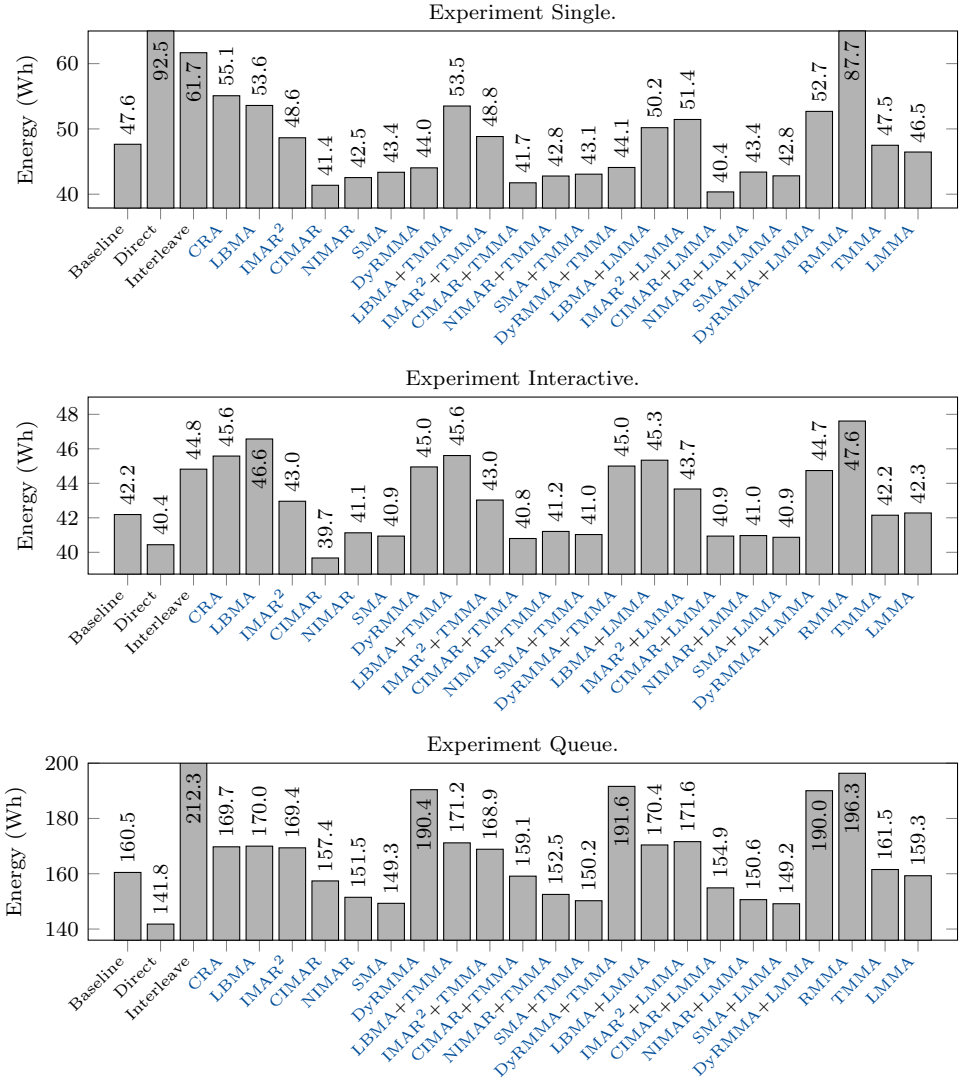
Figure 4.30: Energy (Wh) for Experiments Single, Interactive and Queue in Server ctnuma1. Lower is better.
