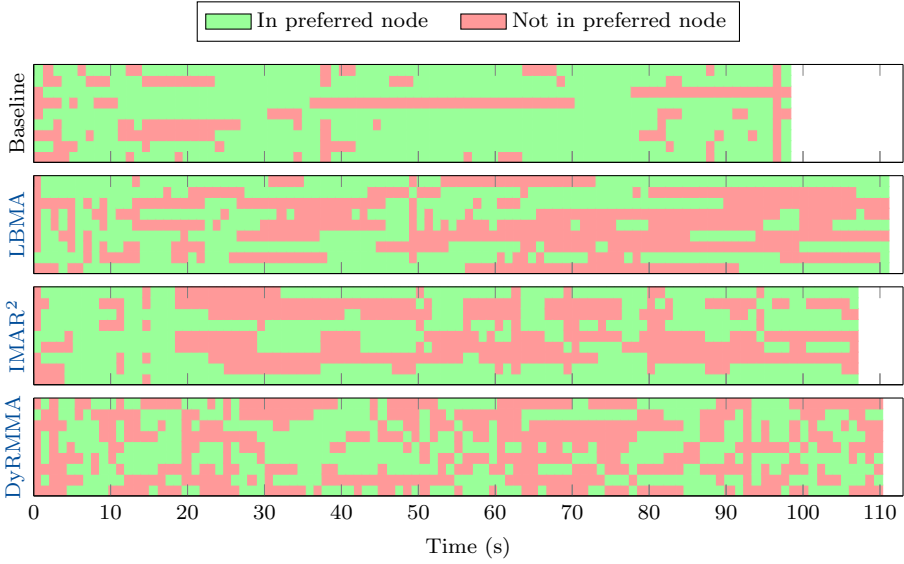
Figure 4.20: Traces showing whether threads are in their preferred node or not for LU.C benchmark running under Baseline, LBMA , IMAR 2 and DyRMMA algorithms in Experiment Queue in Server ctnuma1.
