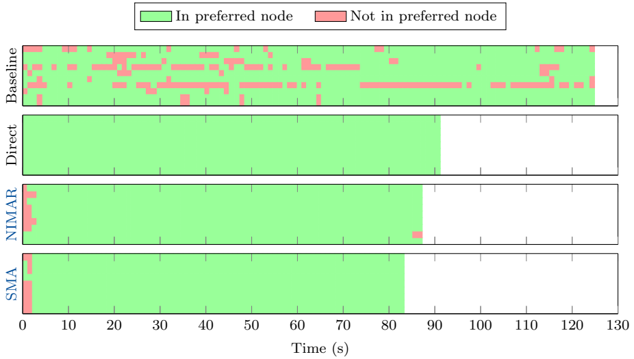
Figure 4.22: Traces showing whether threads are in their preferred node or not for SP.C benchmark running under Baseline, Direct, NIMAR and SMA algorithms in Experiment Queue in Server ctnumal1.
