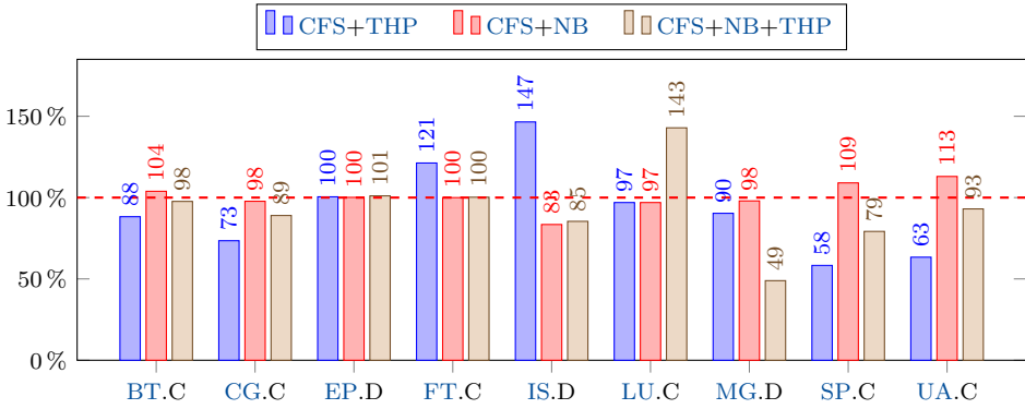
Figure 4.5: Normalised execution times (%) for Experiment Single in Server ctnuma1. Lower is better.
