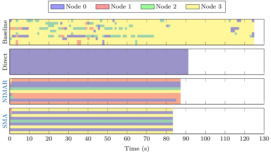
Figure 4.21: Traces showing node in which threads are running for SP.C benchmark running under Baseline, Direct, NIMAR and SMA algorithms in Experiment Queue in Server ctnumal1.
