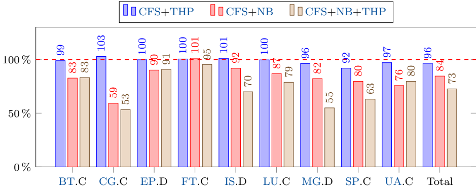
Figure 4.6: Normalised execution times (%) for Experiment Queue in Server ctnuma1. Lower is better.
